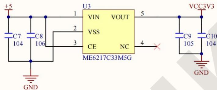
5V to 3.3V voltage regulator circuit
