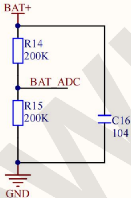
Battery level detection circuit
